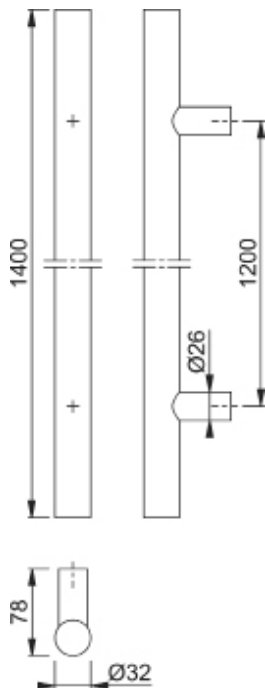
1400mm bar length
