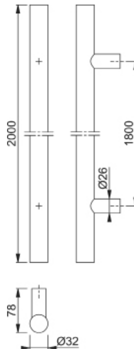
2000mm bar length
